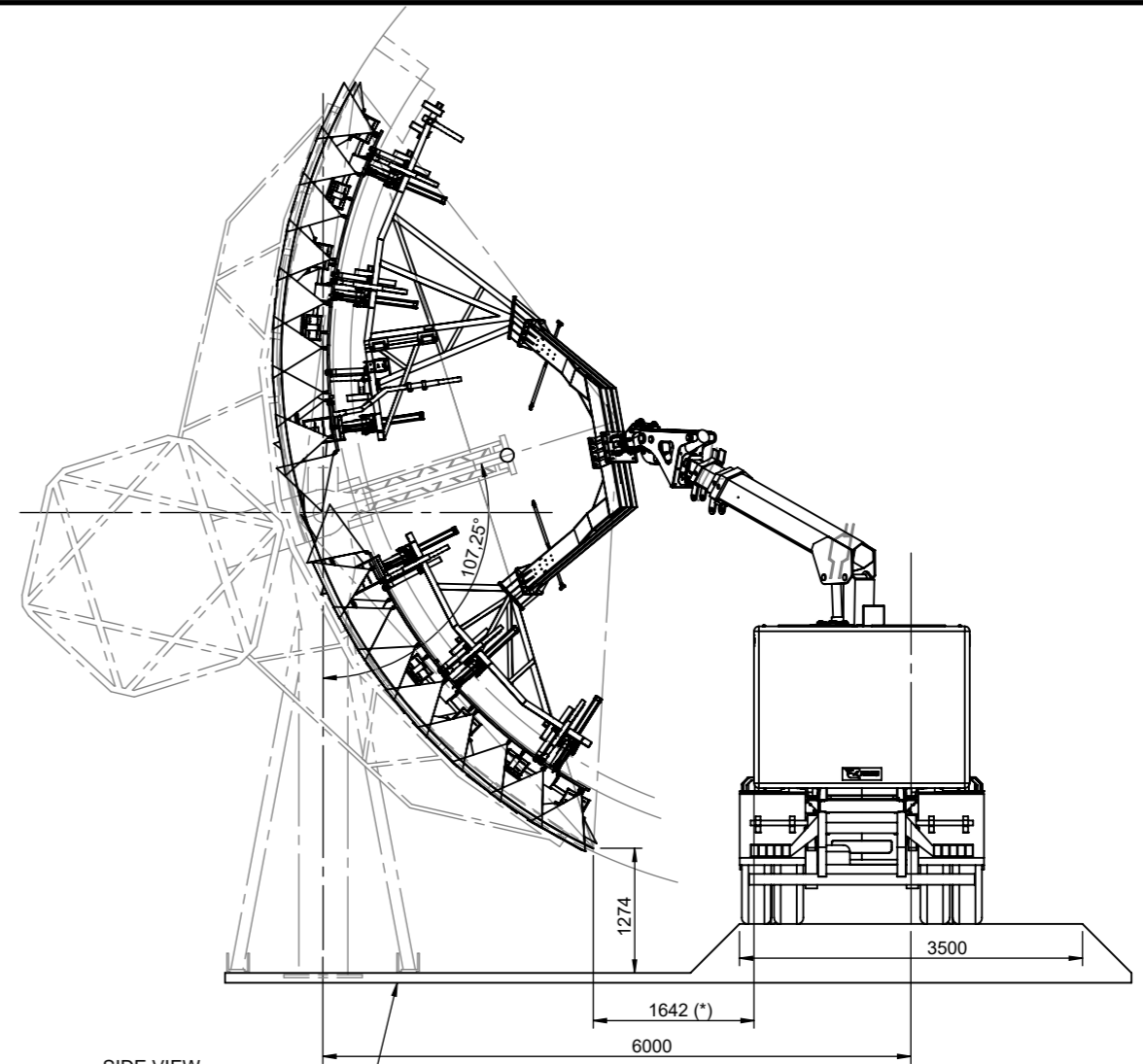
SIDE VIEW
