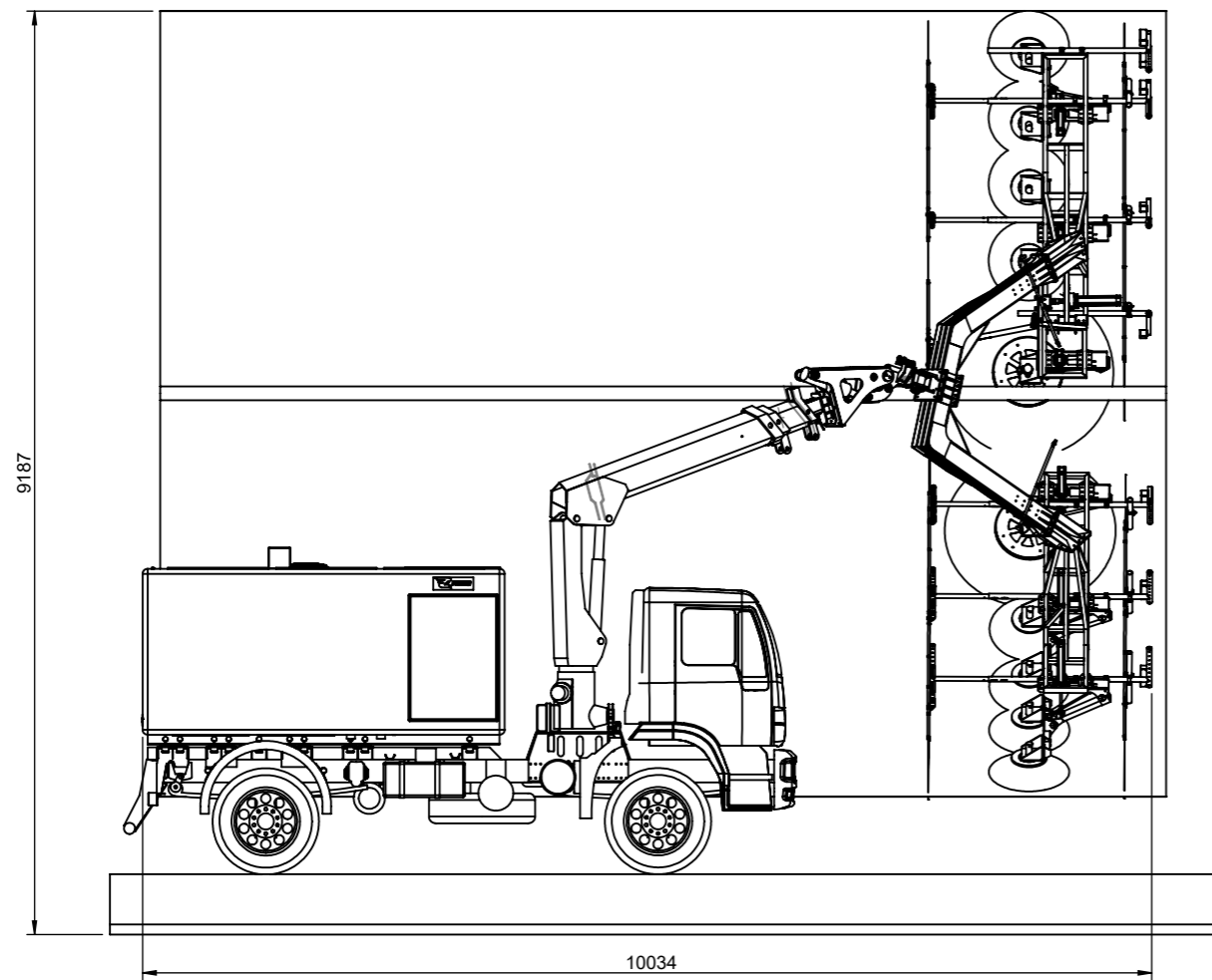
FRONT VIEW
